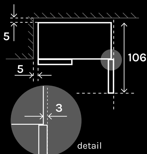
Doors opening dimensions (cm)
